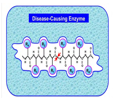
Figure 1: A schematic illustration to show a peptide in good fitting and tightly binding with the enzyme's active site before it is cleaved by the latter. Adapted from [296] with permission.
