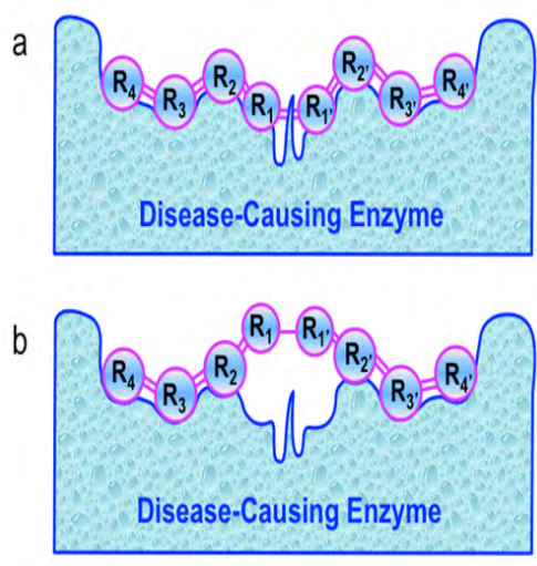
Figure 2: Schematic drawing to illustrate the "Distorted Key" theory, where panel
